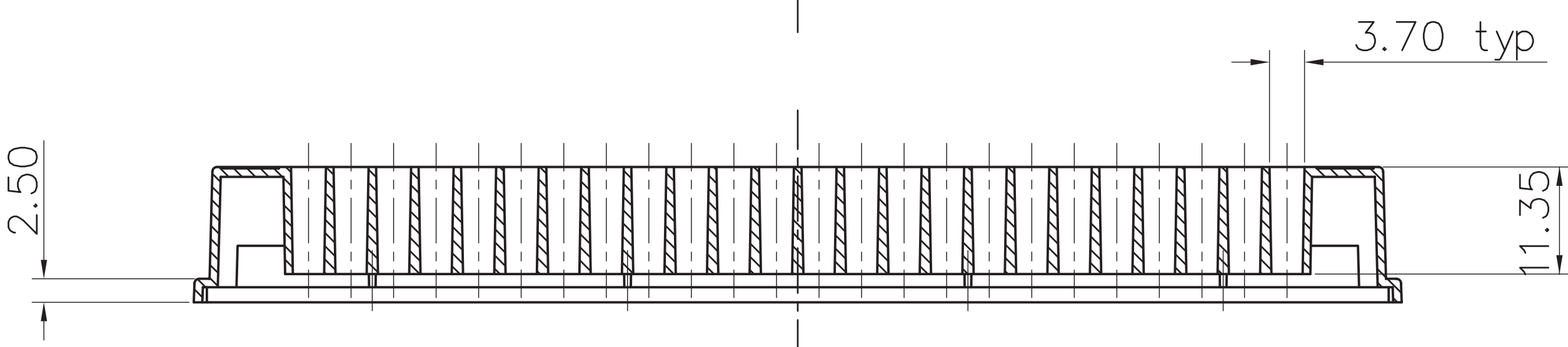
SECTION X-X
